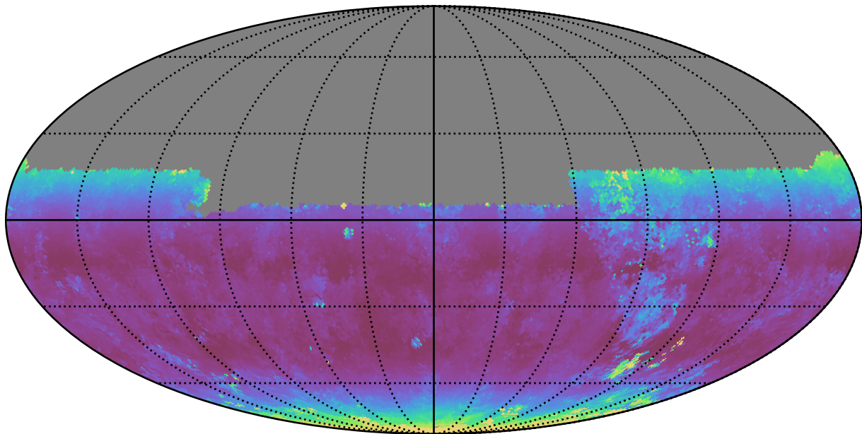
scp_reweight_v3.3_10yrs Yr 1 y band: Median airmass
