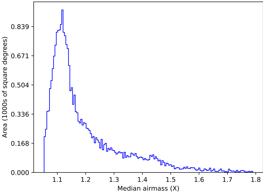
scp_reweight_v3.3_10yrs Yr 1 y band: Median airmass
