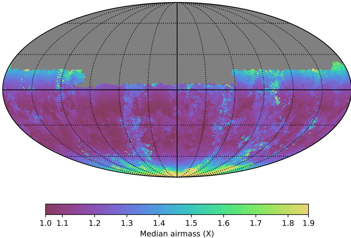
scp_reweight_v3.3_10yrs Yr 1 u band: Median airmass
