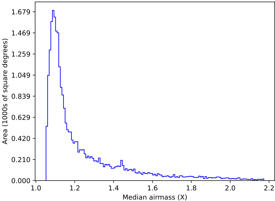
scp_reweight_v3.3_10yrs Yr 1 i band: Median airmass
