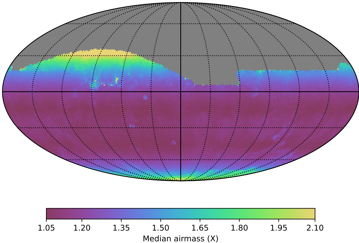
scp_reweight_v3.3_10yrs Yr 1 all bands: Median airmass
