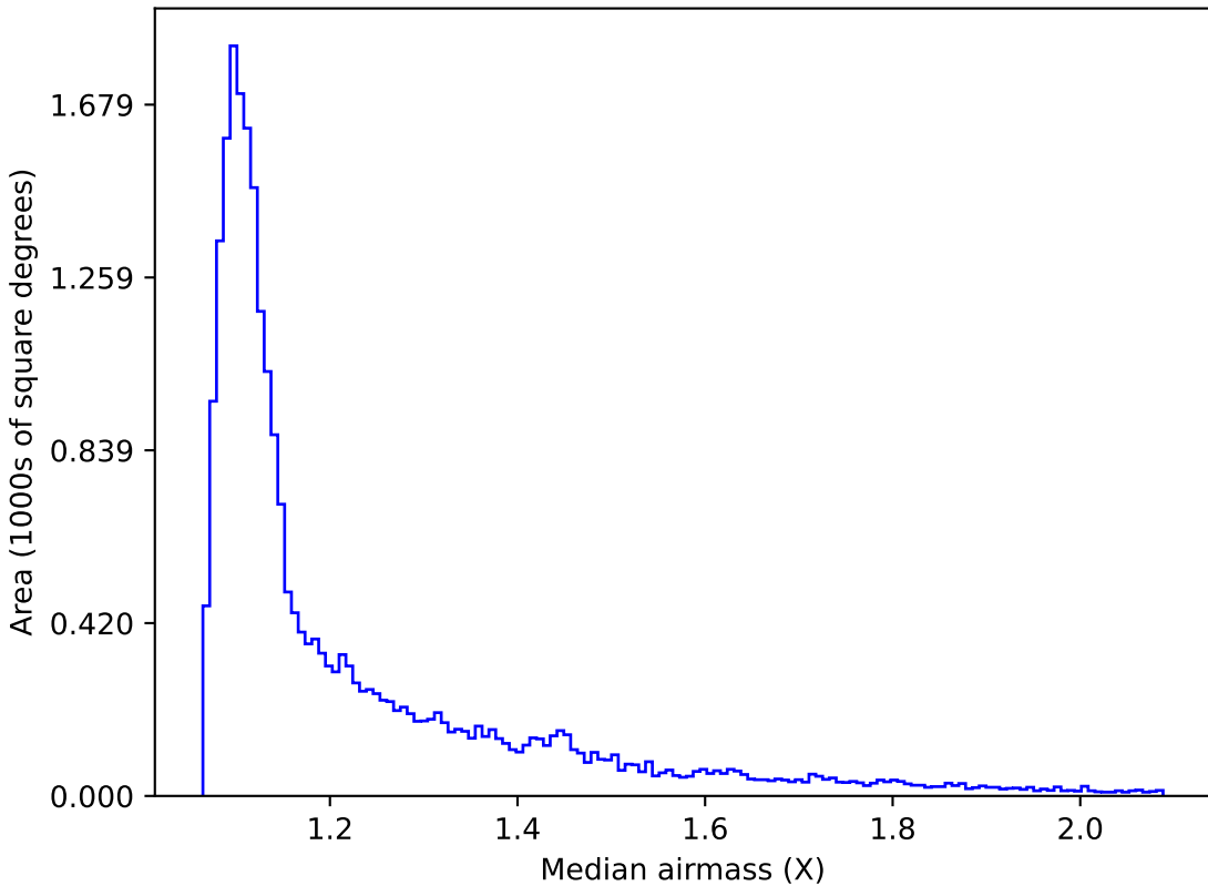
scp_reweight_v3.3_10yrs Yr 1 all bands: Median airmass
