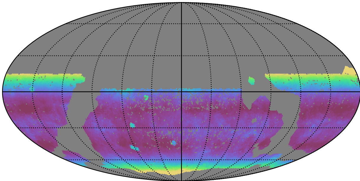
scp_reweight_v3.3_10yrs WFD z band: Median airmass
