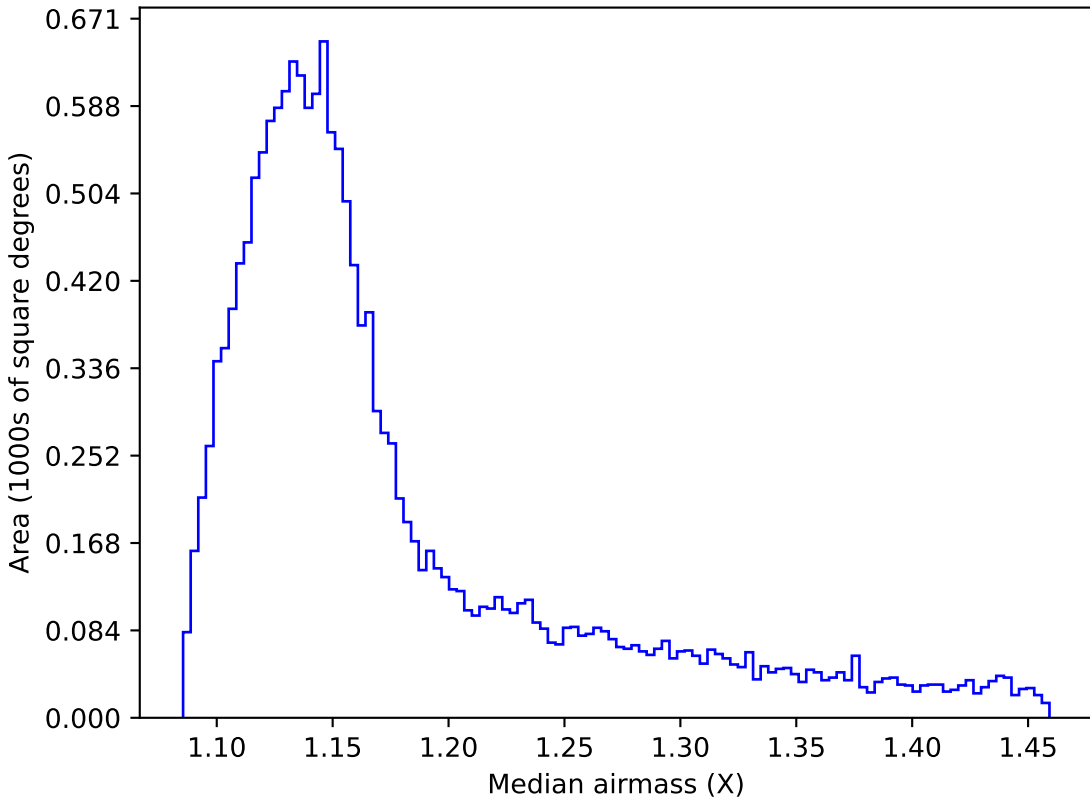
scp_reweight_v3.3_10yrs WFD z band: Median airmass
