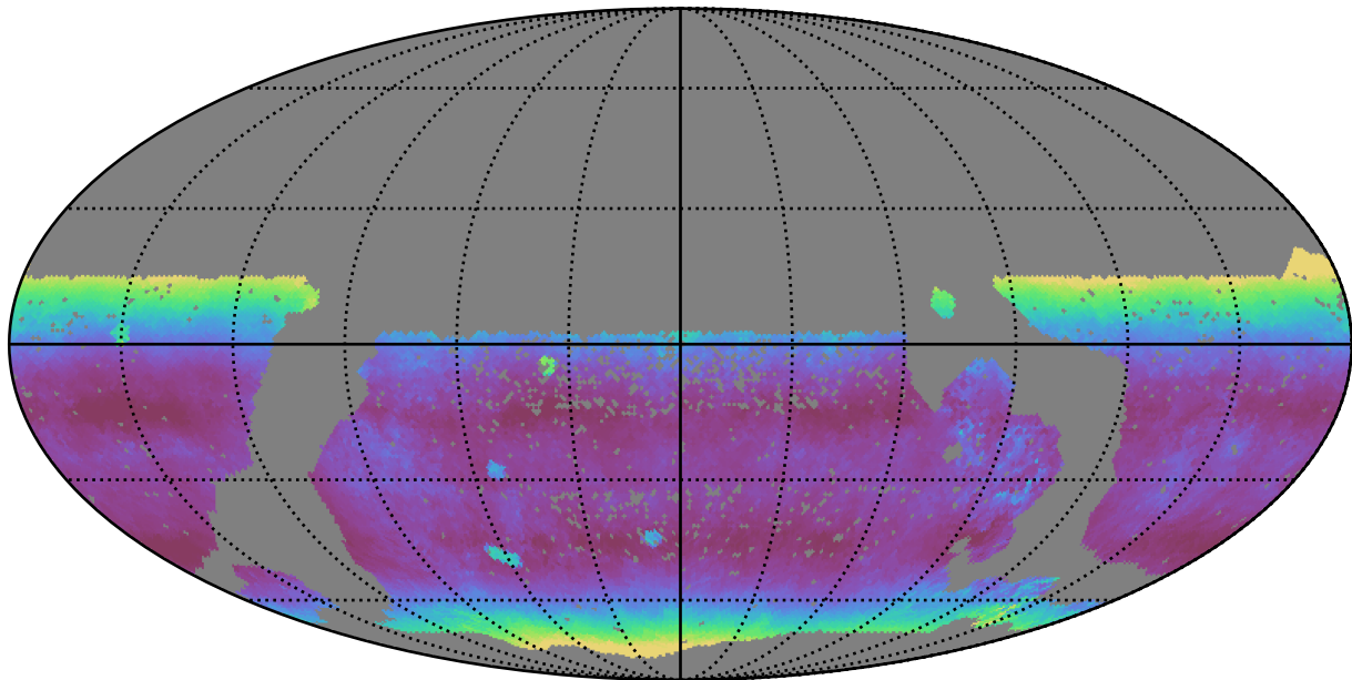
scp_reweight_v3.3_10yrs WFD y band: Median airmass
