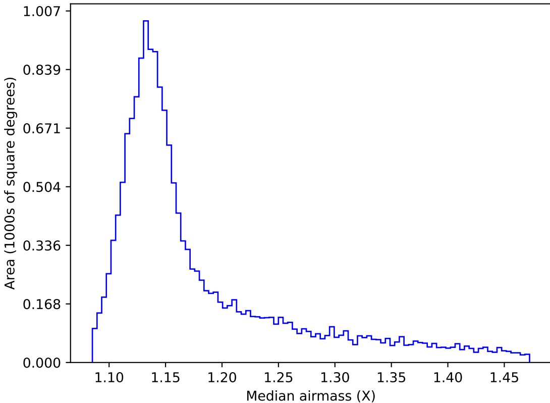
scp_reweight_v3.3_10yrs WFD y band: Median airmass
