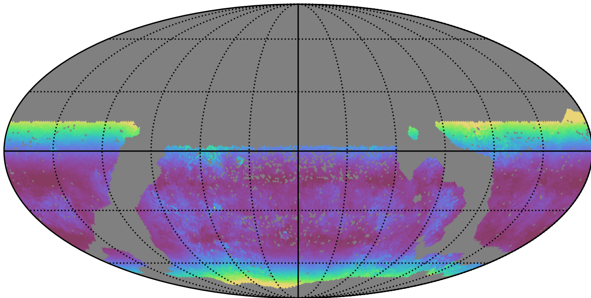
scp_reweight_v3.3_10yrs WFD u band: Median airmass
