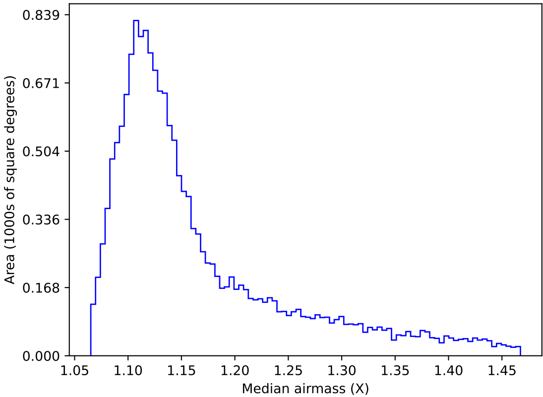
scp_reweight_v3.3_10yrs WFD u band: Median airmass
