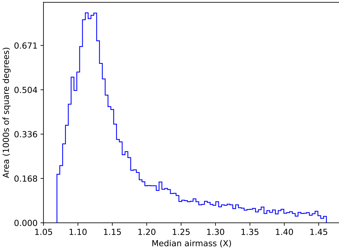
scp_reweight_v3.3_10yrs WFD r band: Median airmass
