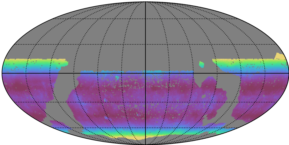
scp_reweight_v3.3_10yrs WFD i band: Median airmass
