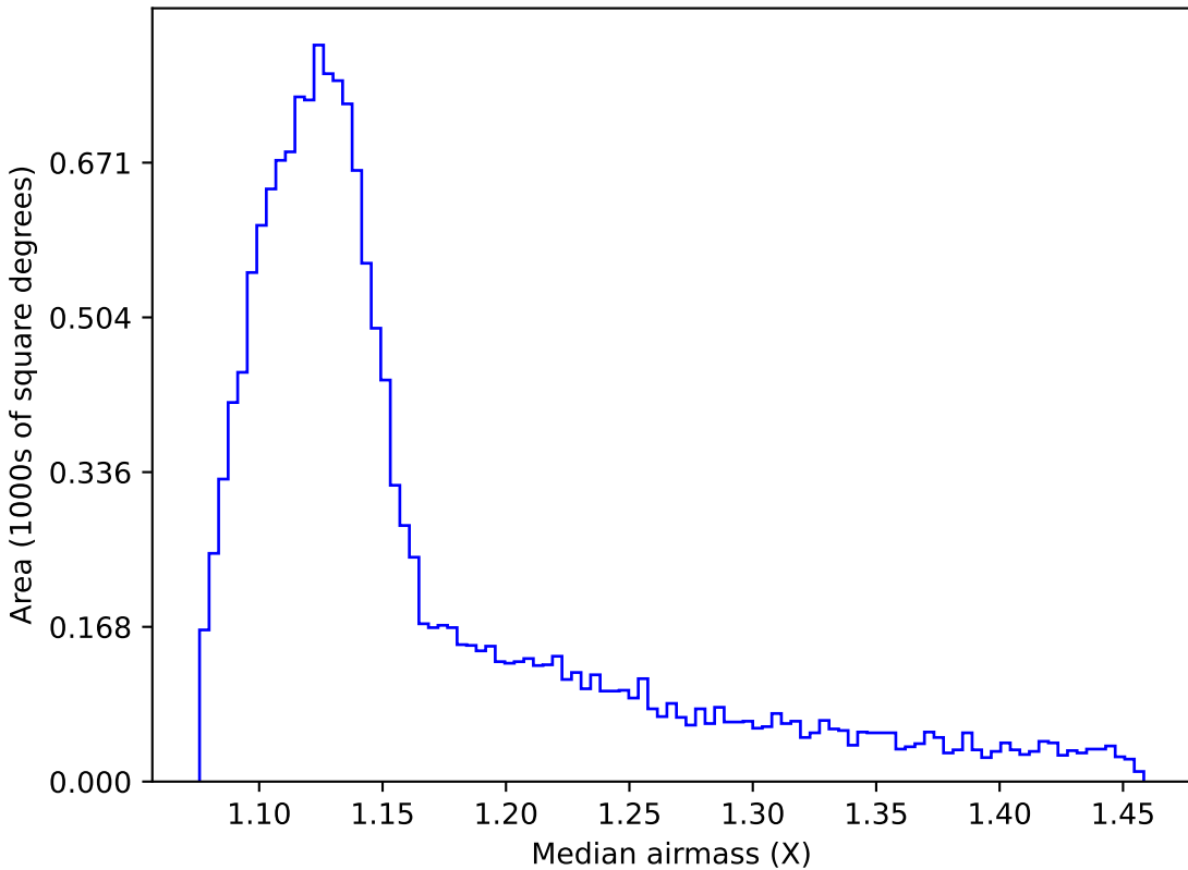
scp_reweight_v3.3_10yrs WFD i band: Median airmass
