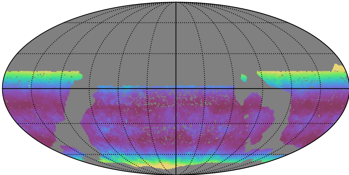
scp_reweight_v3.3_10yrs WFD g band: Median airmass
