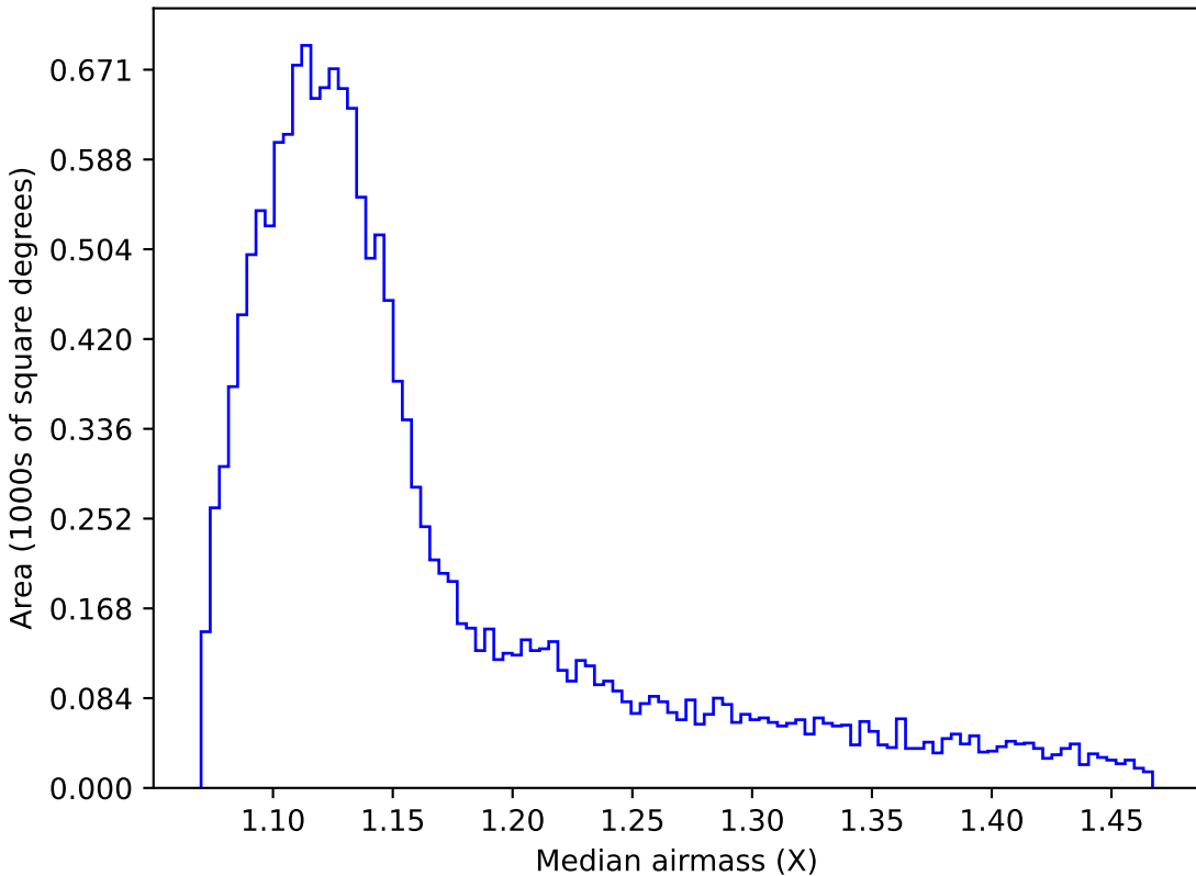
scp_reweight_v3.3_10yrs WFD g band: Median airmass
