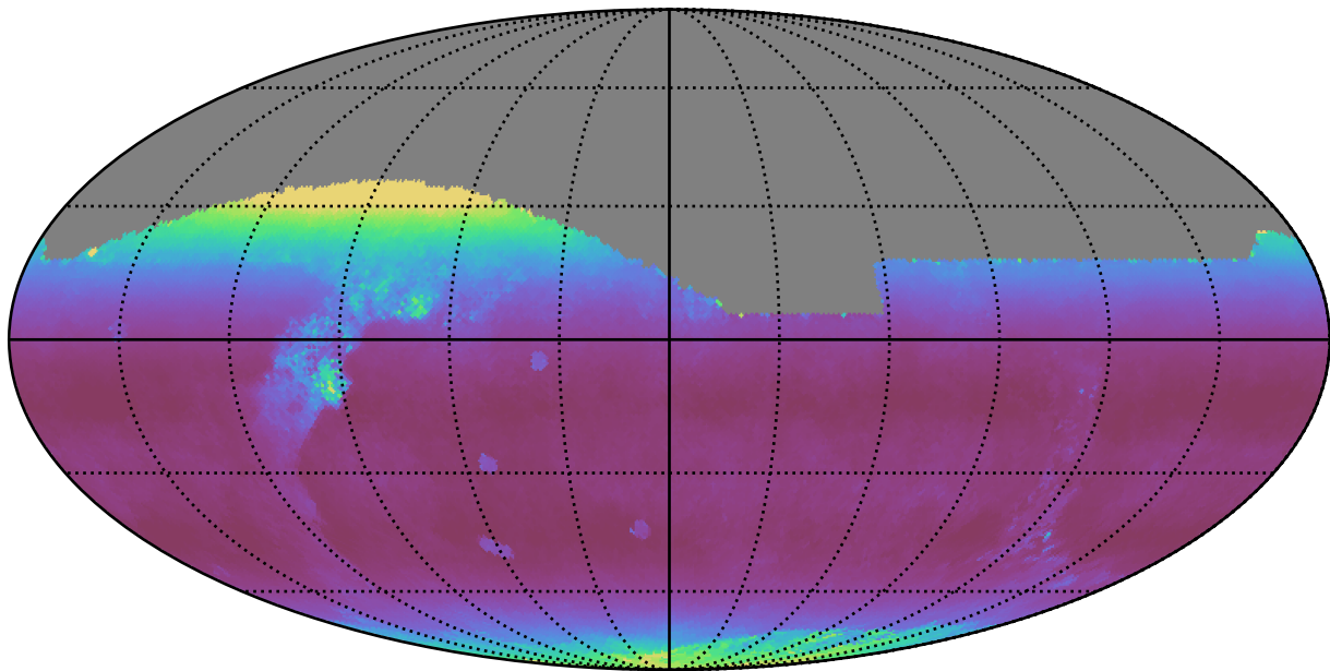
scp_reweight_v3.3_10yrs All sky z band: Median airmass
