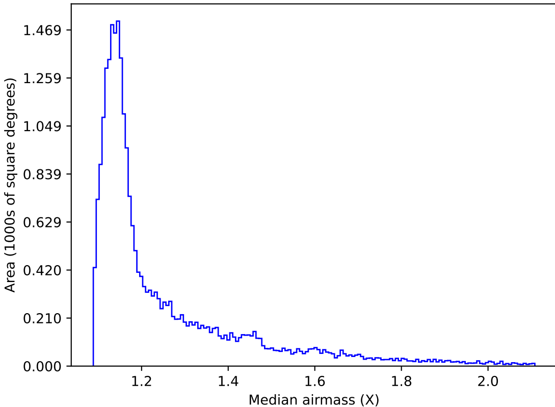
scp_reweight_v3.3_10yrs All sky z band: Median airmass
