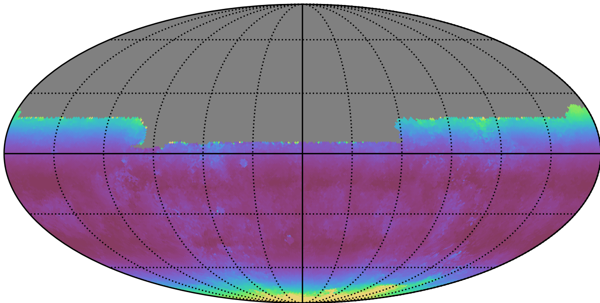
scp_reweight_v3.3_10yrs All sky u band: Median airmass
