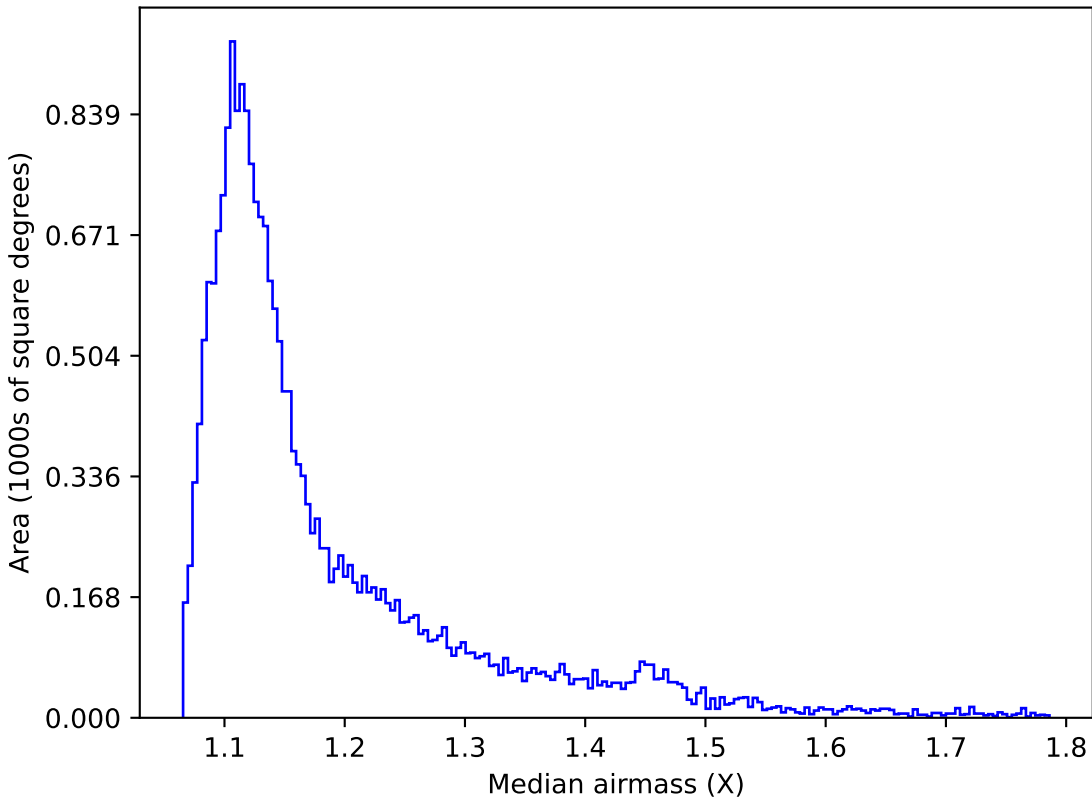
scp_reweight_v3.3_10yrs All sky u band: Median airmass
