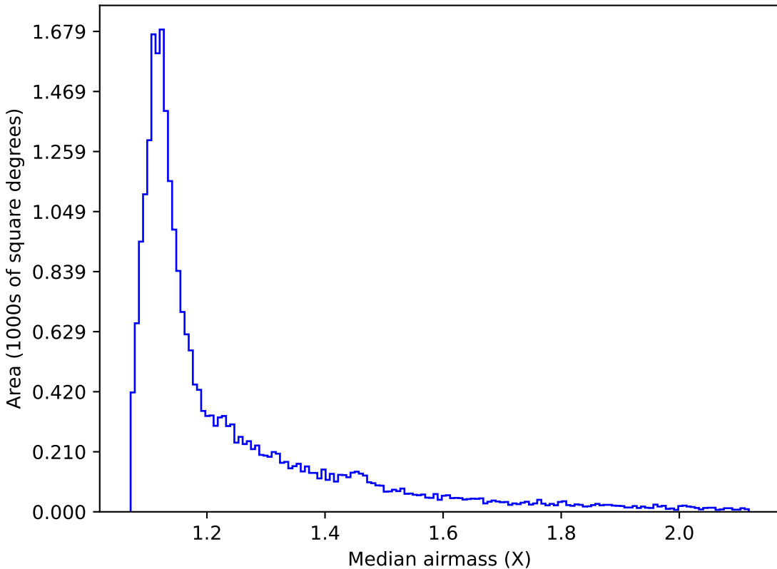
scp_reweight_v3.3_10yrs All sky r band: Median airmass
