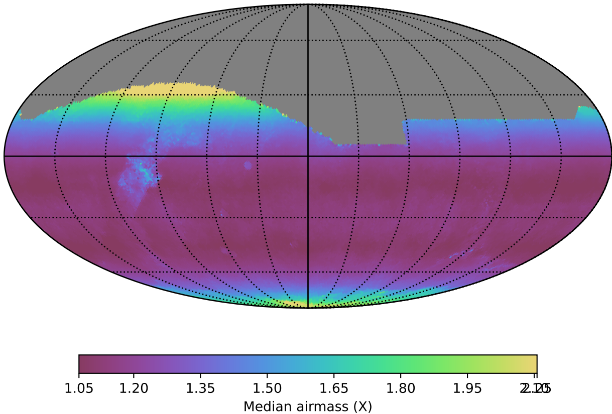
scp_reweight_v3.3_10yrs All sky i band: Median airmass
