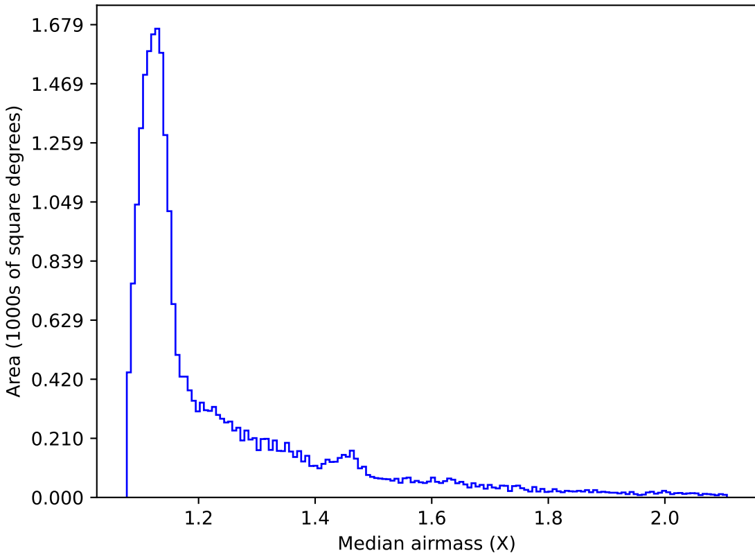
scp_reweight_v3.3_10yrs All sky i band: Median airmass
