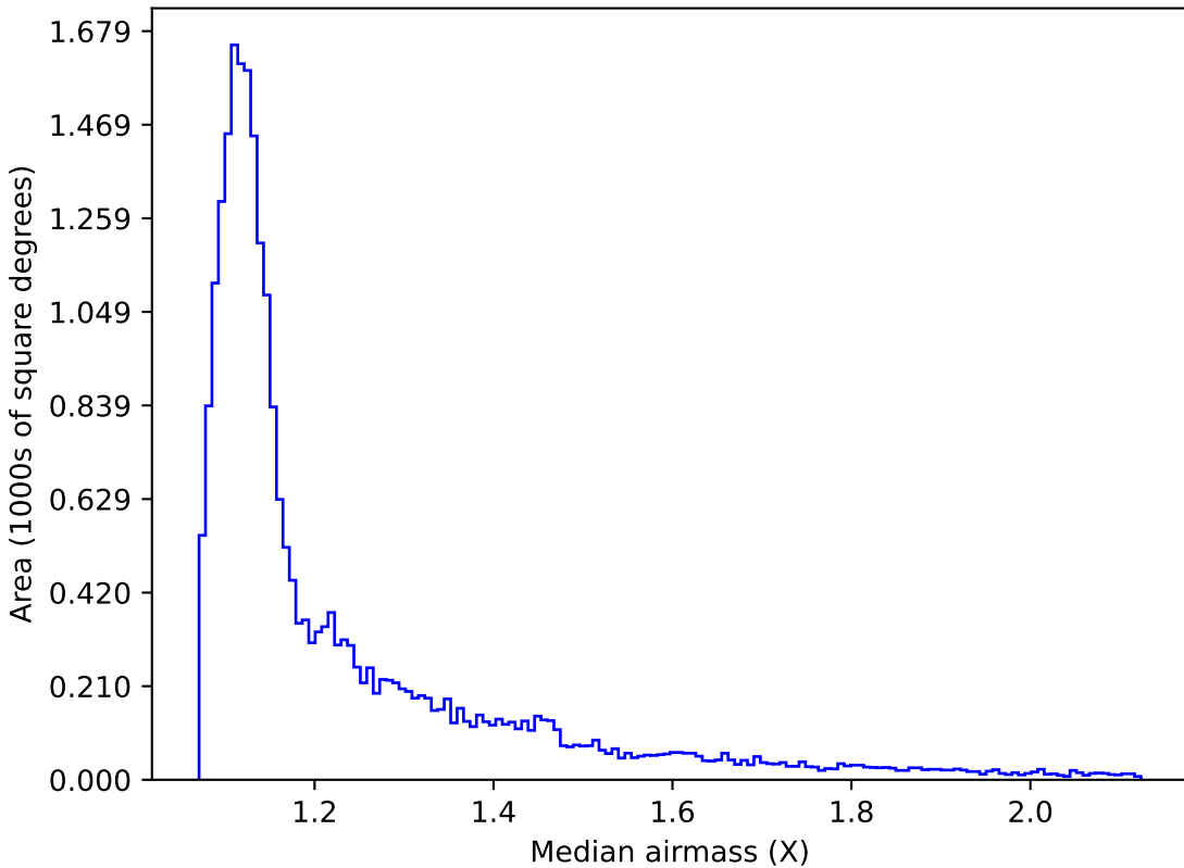
scp_reweight_v3.3_10yrs All sky g band: Median airmass
