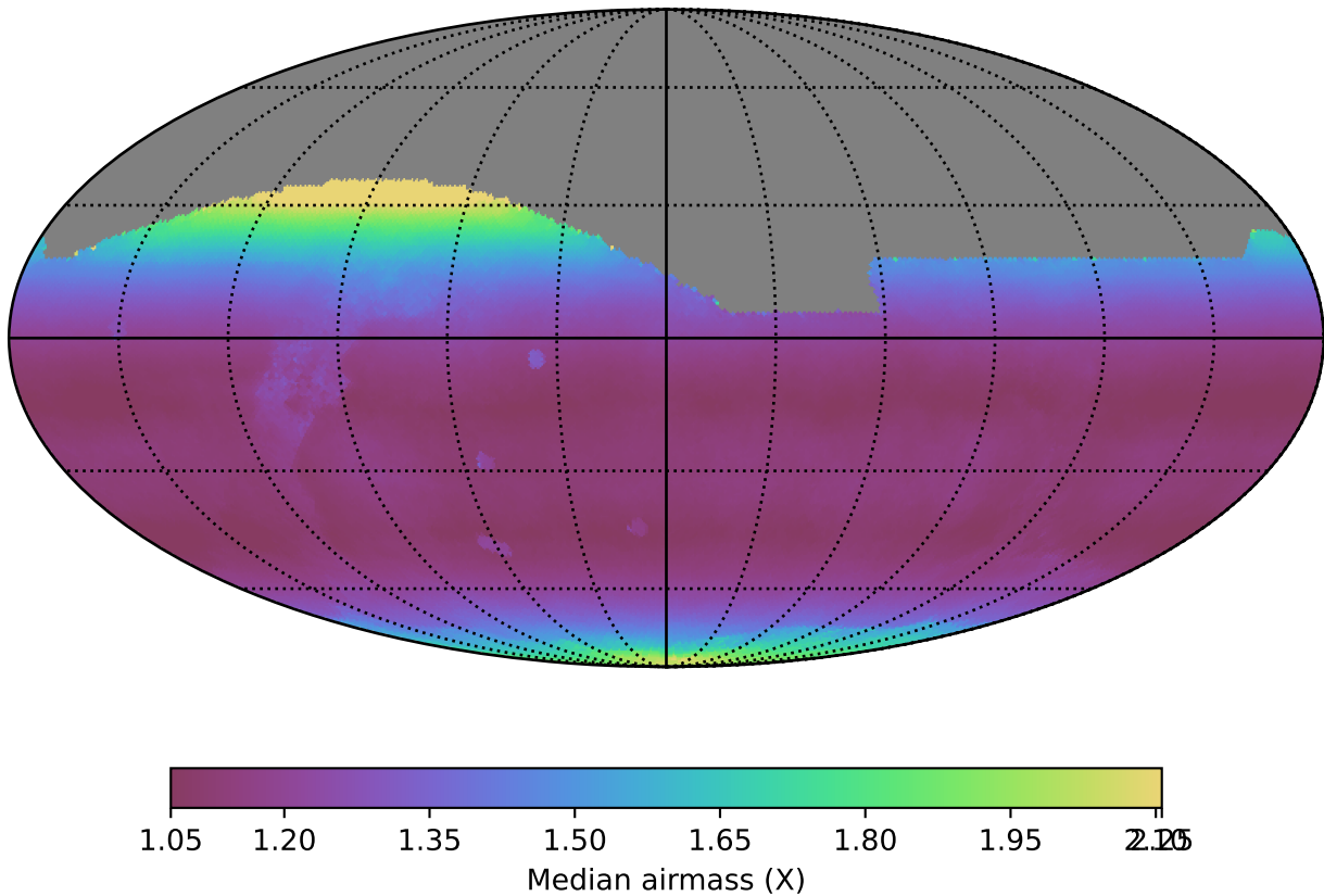
scp_reweight_v3.3_10yrs All sky all bands: Median airmass
