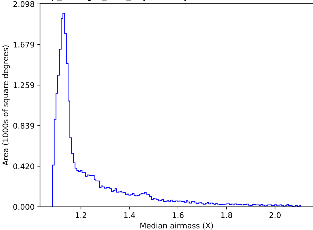
scp_reweight_v3.3_10yrs All sky all bands: Median airmass
