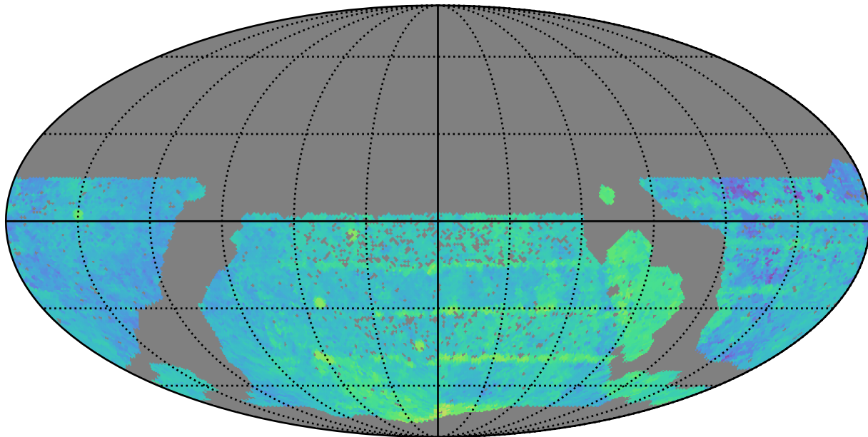
scp_reweight_v3.3_10yrs WFD z band: Median Season Length
