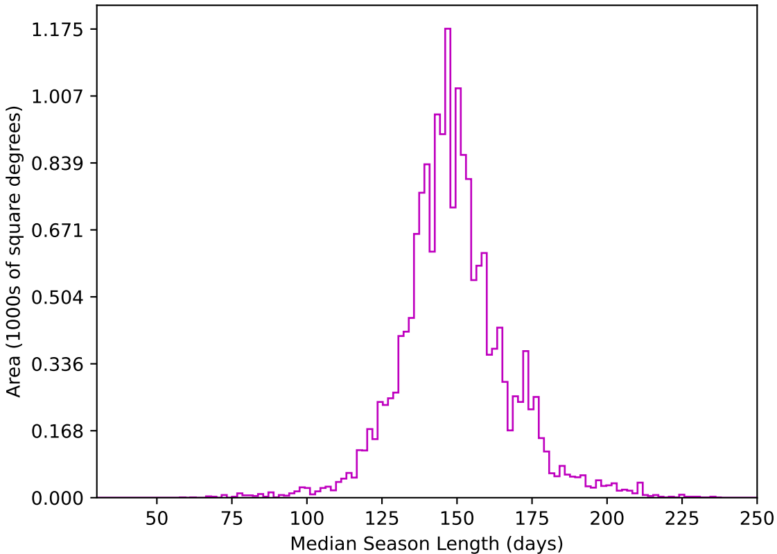
scp_reweight_v3.3_10yrs WFD z band: Median Season Length
