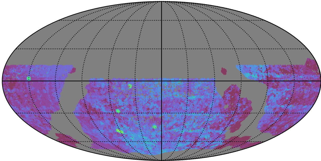
scp_reweight_v3.3_10yrs WFD u band: Median Season Length
