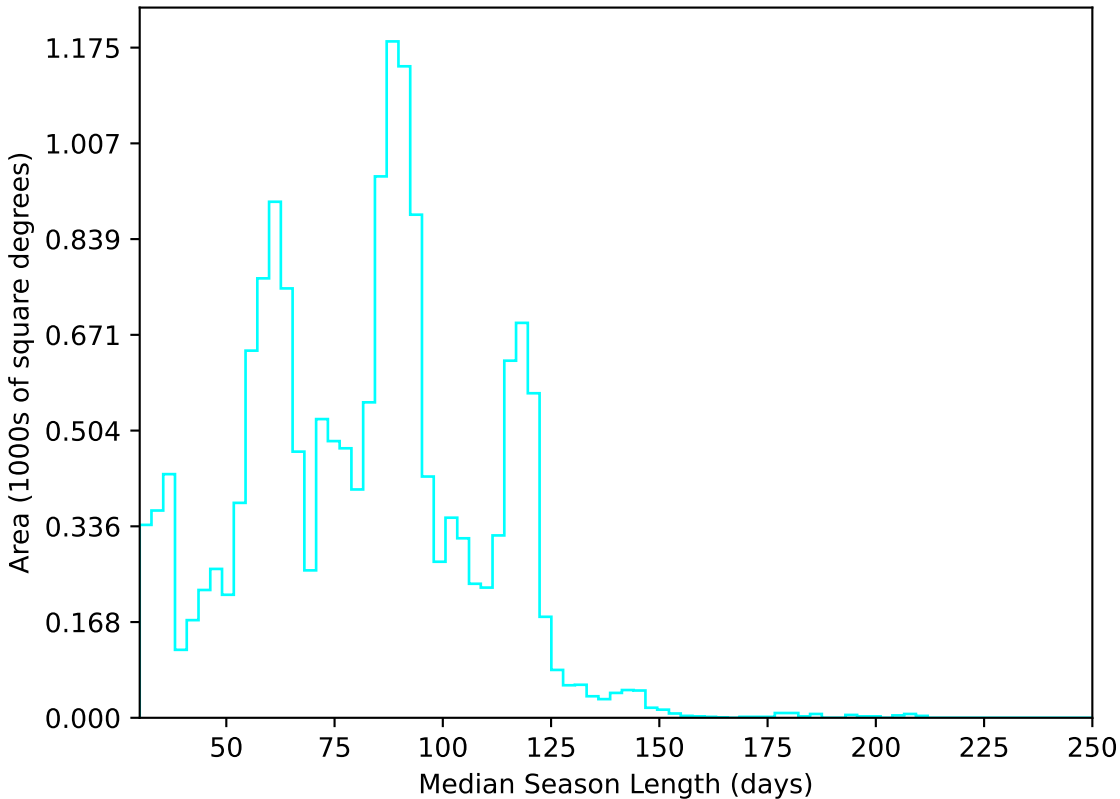
scp_reweight_v3.3_10yrs WFD u band: Median Season Length
