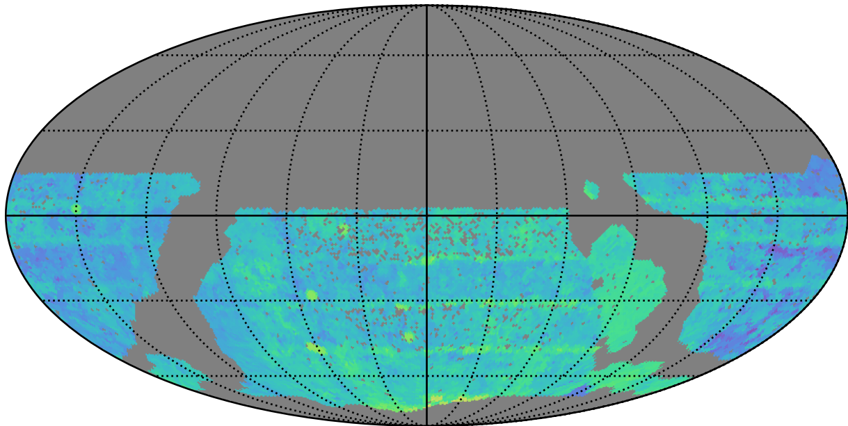
scp_reweight_v3.3_10yrs WFD r band: Median Season Length
