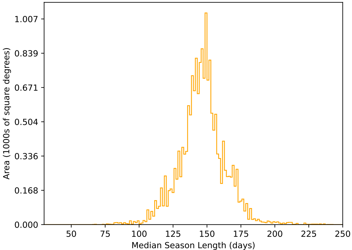
scp_reweight_v3.3_10yrs WFD r band: Median Season Length
