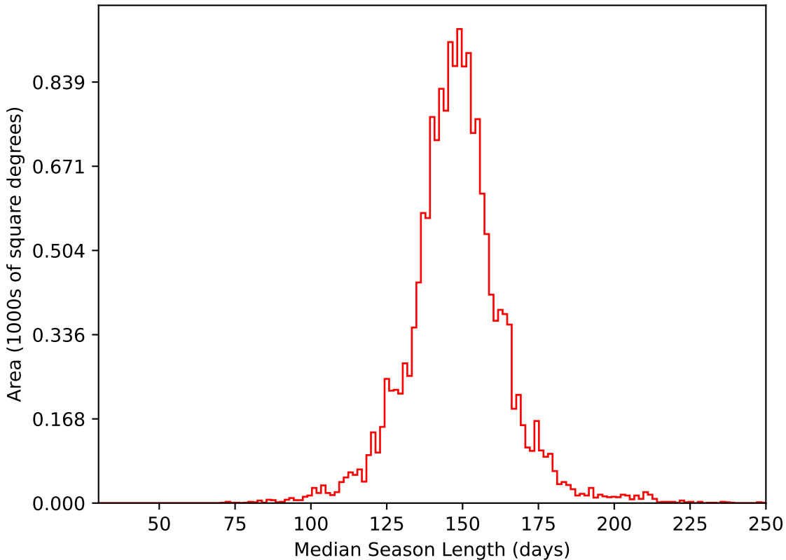
scp_reweight_v3.3_10yrs WFD i band: Median Season Length
