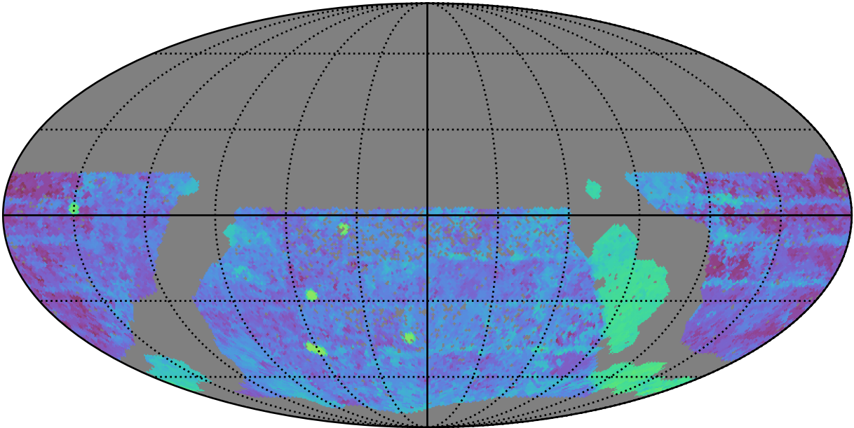
scp_reweight_v3.3_10yrs WFD g band: Median Season Length
