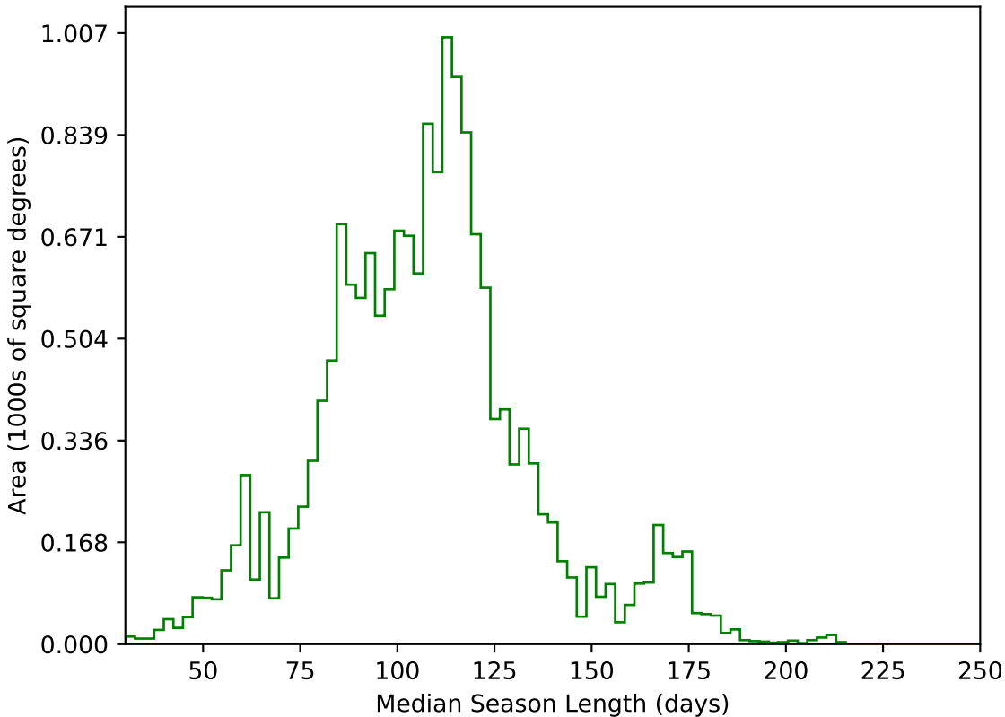
scp_reweight_v3.3_10yrs WFD g band: Median Season Length
