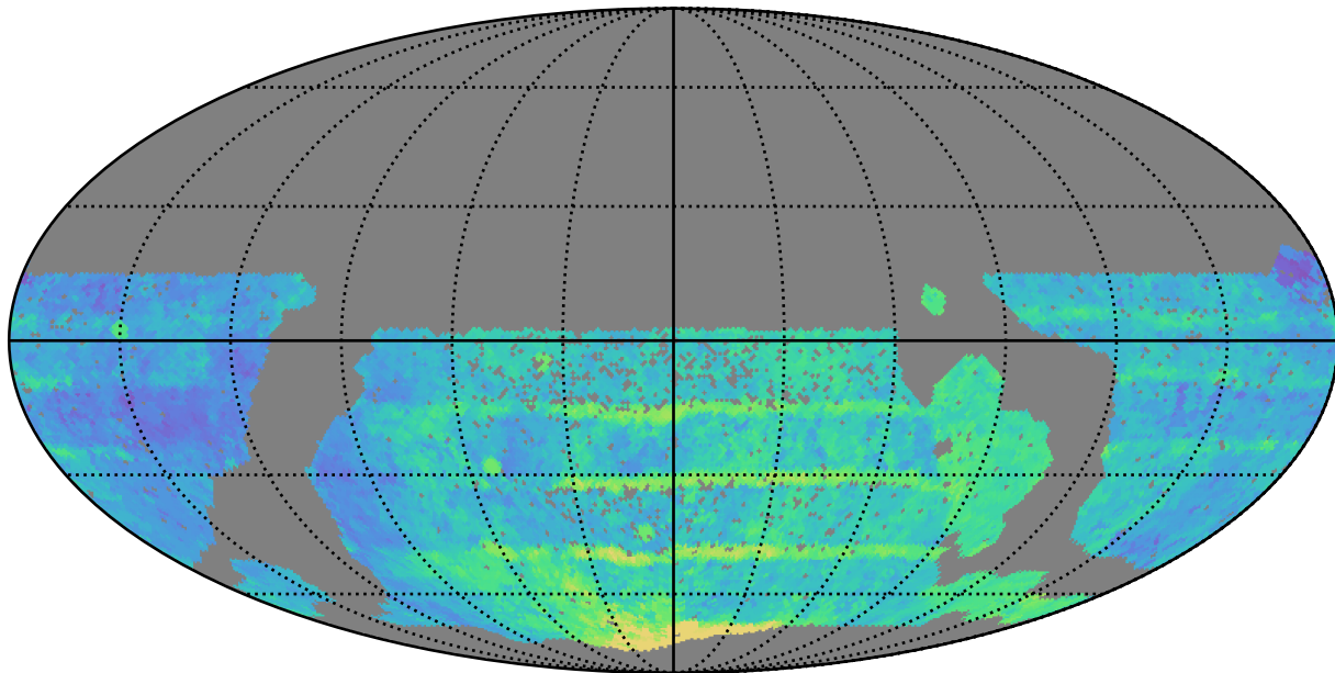
scp_reweight_v3.3_10yrs WFD all bands: Median Season Length
