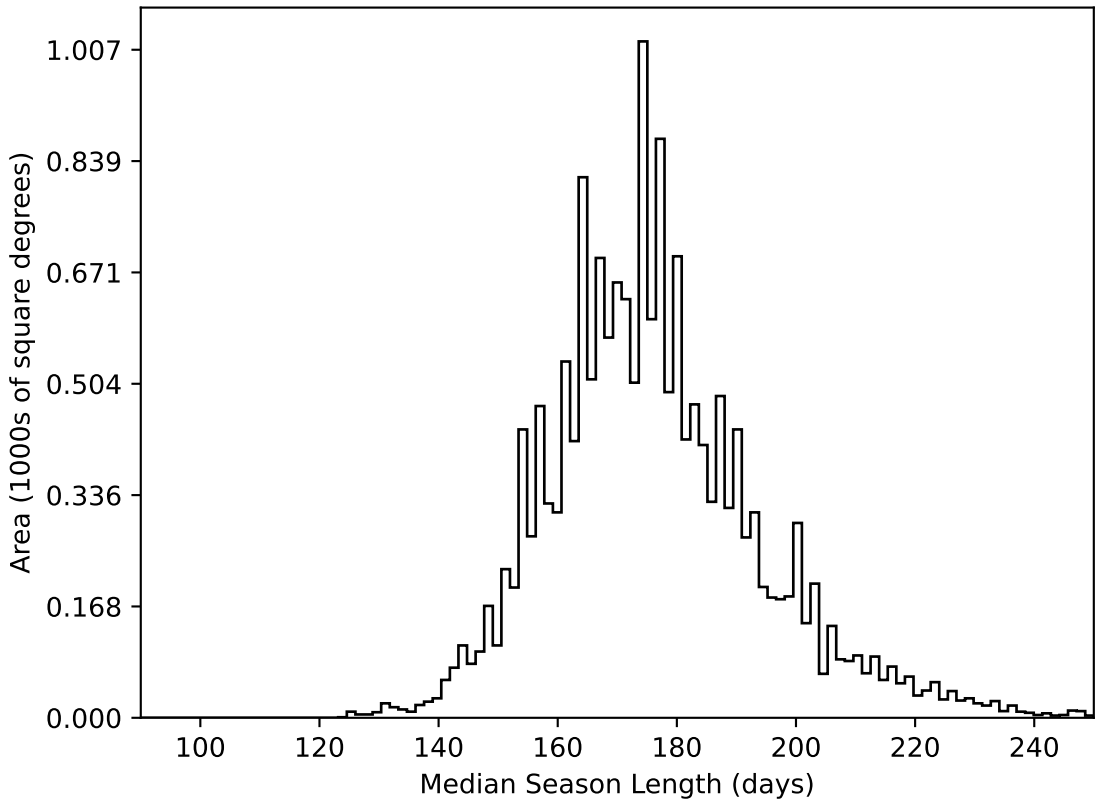
scp_reweight_v3.3_10yrs WFD all bands: Median Season Length
