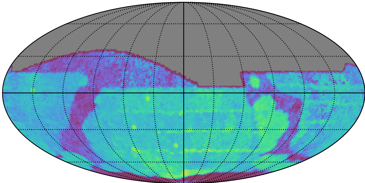
scp_reweight_v3.3_10yrs All sky z band: Median Season Length
