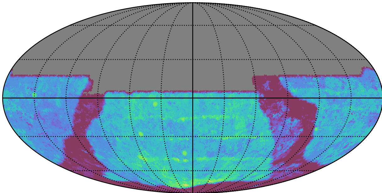
scp_reweight_v3.3_10yrs All sky y band: Median Season Length
