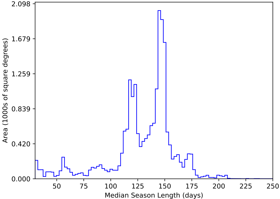
scp_reweight_v3.3_10yrs All sky y band: Median Season Length
