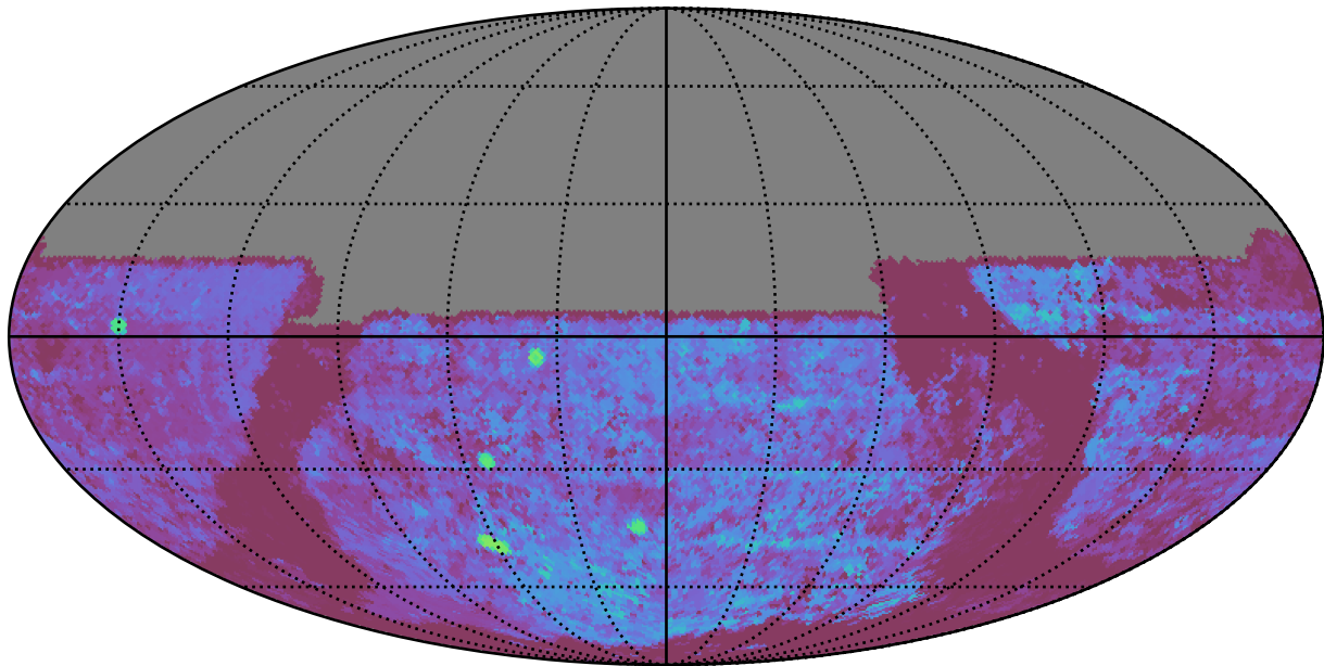
scp_reweight_v3.3_10yrs All sky u band: Median Season Length
