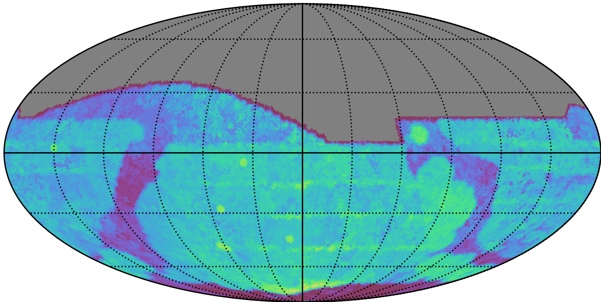
scp_reweight_v3.3_10yrs All sky i band: Median Season Length
