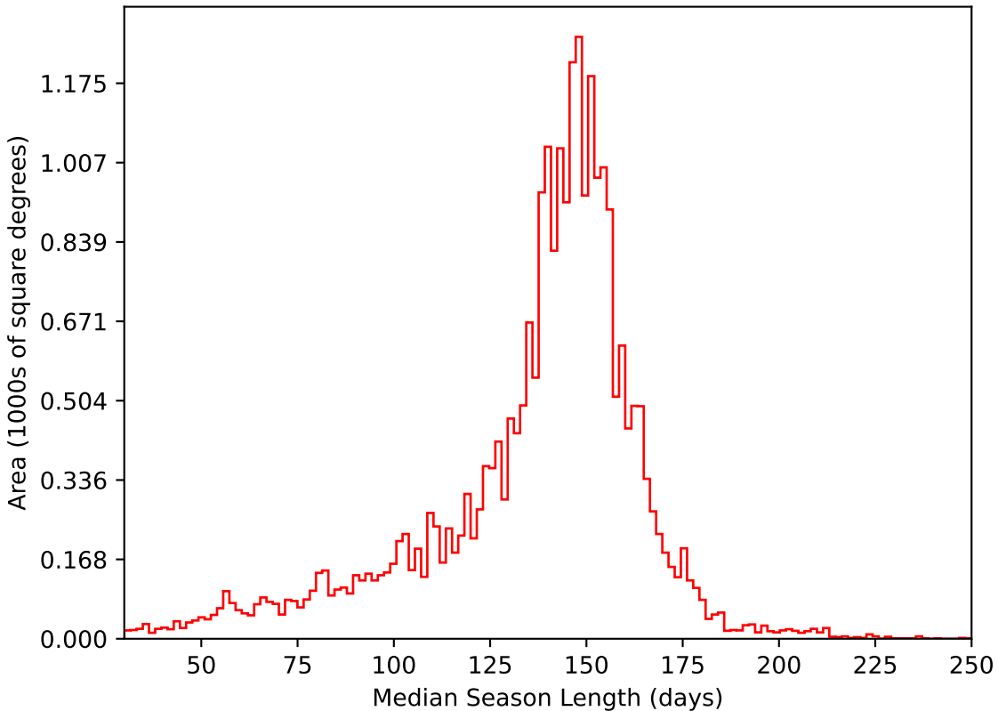
scp_reweight_v3.3_10yrs All sky i band: Median Season Length
