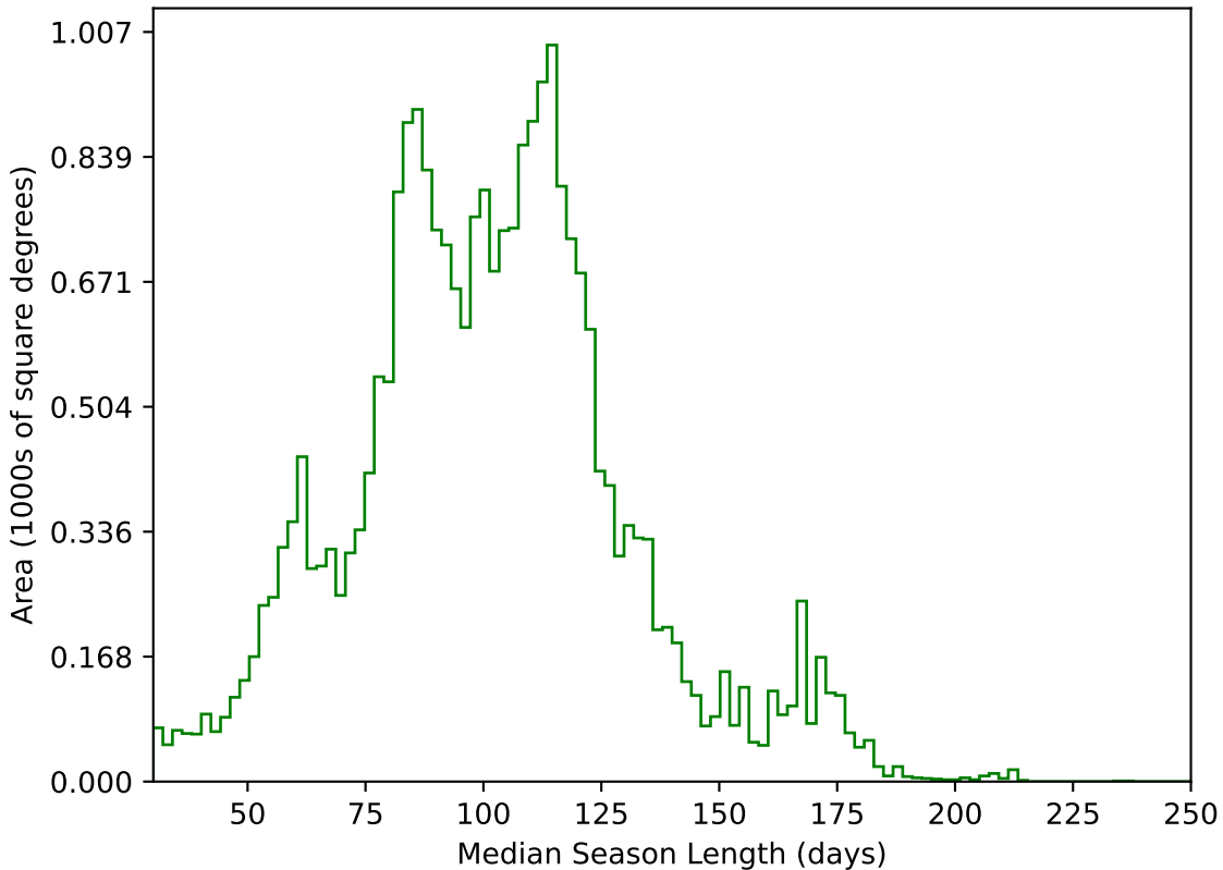
scp_reweight_v3.3_10yrs All sky g band: Median Season Length
