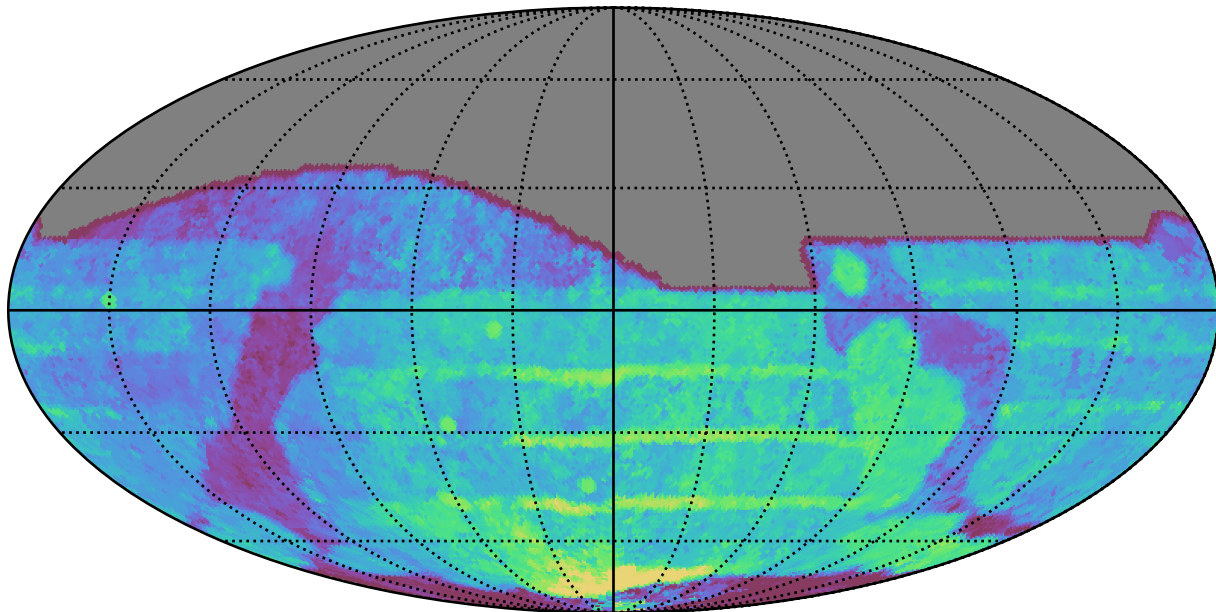
scp_reweight_v3.3_10yrs All sky all bands: Median Season Length
