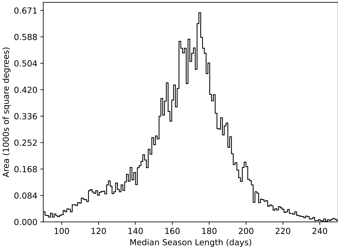
scp_reweight_v3.3_10yrs All sky all bands: Median Season Length
