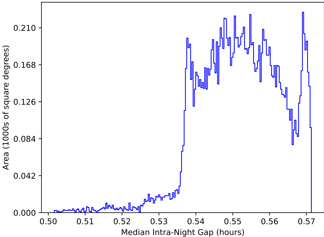
scp_reweight_v3.3_10yrs WFD: Median Intra-Night Gap
