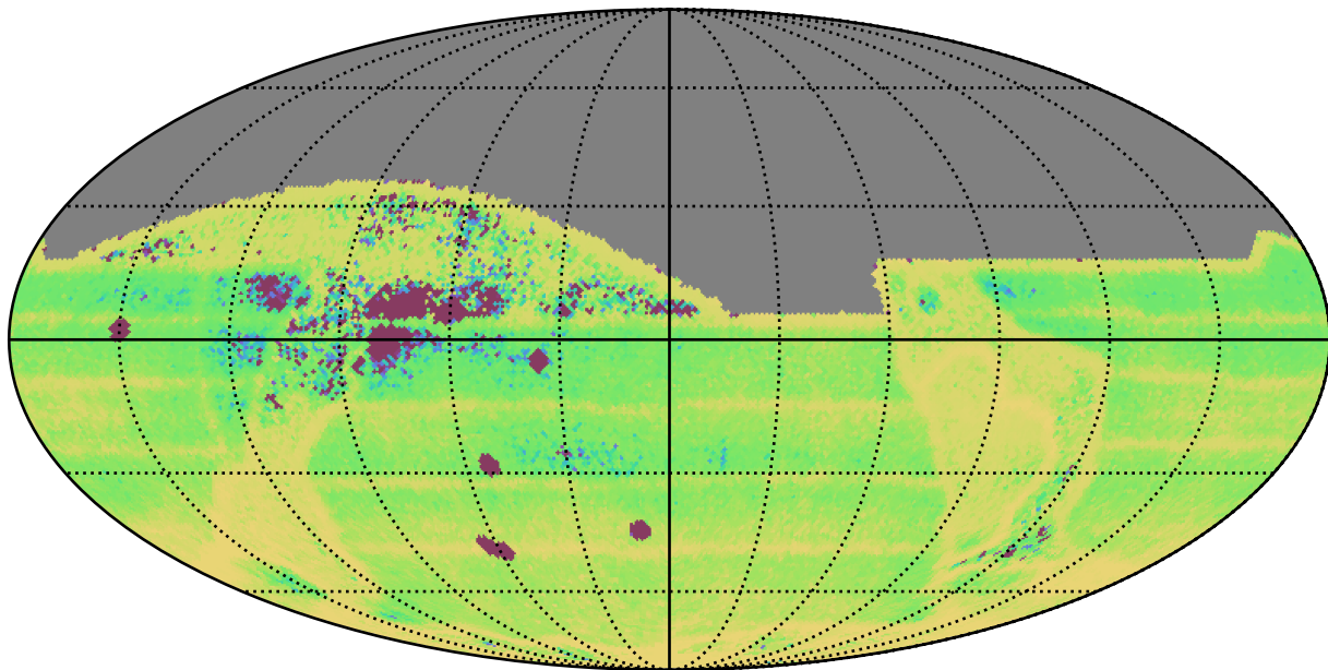
scp_reweight_v3.3_10yrs All sky: Median Intra-Night Gap
