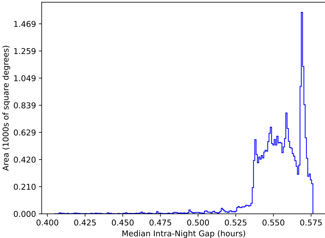
scp_reweight_v3.3_10yrs All sky: Median Intra-Night Gap
